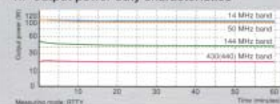
• RF output power duty characteristics
